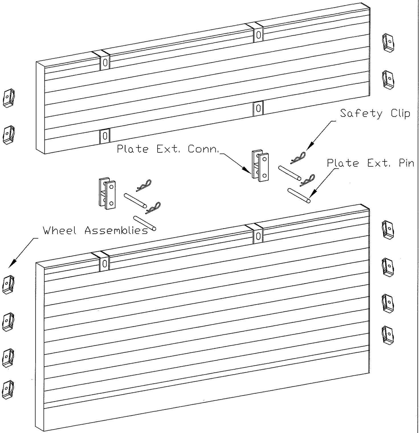
Base Plate and Ext Plate Connection Details
